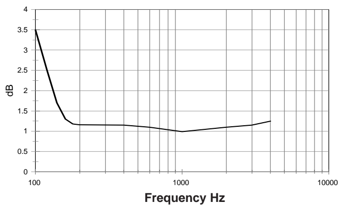
Insertion Loss Typical
